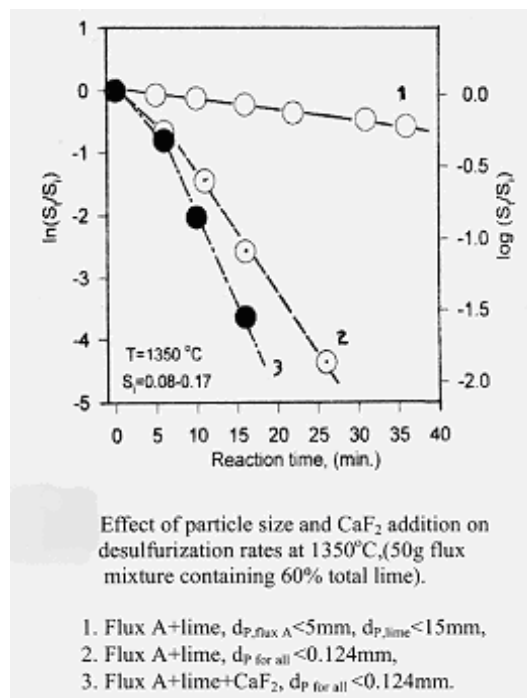
Fig. 3 Effect of particle size and additions on desulfurization rates.
