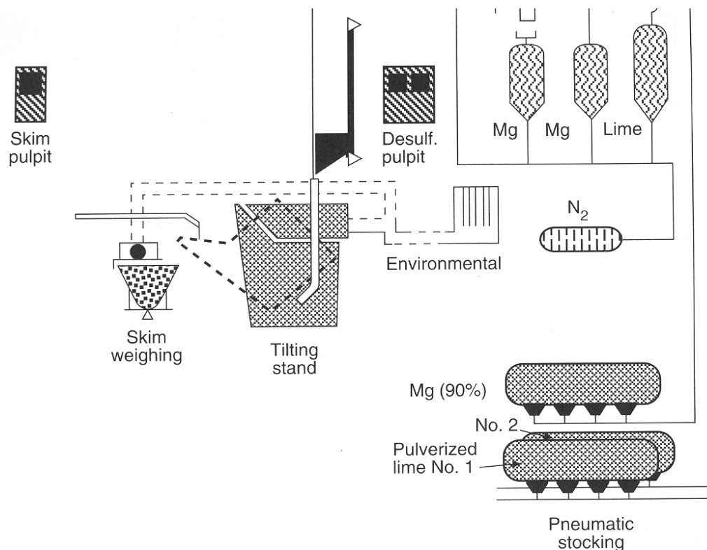
Fig. 1 Diagram of hot metal treatment station using co-injection technology – LTV
