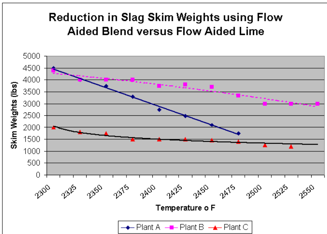
Fig. 5. Graph of trial plants showing reduction in amount of slag skimmed using "flow aided blend" as compared to the prior art material (flow aided lime).
