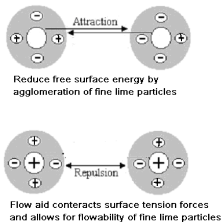
Fig. 4 Flow aided ingredient influences electrical charges on the particles to repel other particles.
