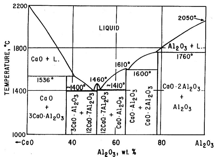
Fig. 2 Phase-equilibrium diagram for CaO-Al 2 O 3 system.
